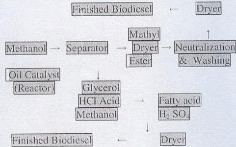
Fig.2: Schematic of Biodiesel Processing.
