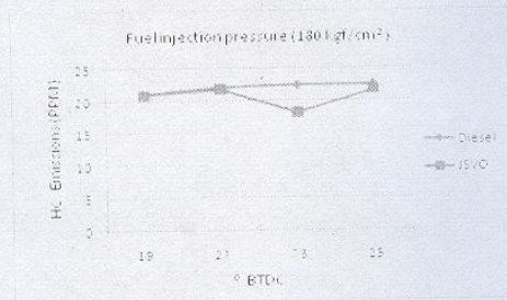
Figure 11: HC emissions of Diesel & JSVO fuel with various fuel injection pressures at different 0 BTDC Fuel injection advance angles.
