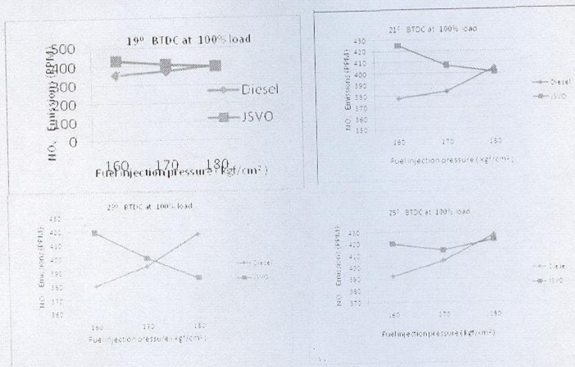
Figure 10: NO x emissions of Diesel & JSVO fuel with various fuel injection pressures at different 0 BTDC Fuel injection advance angles.
